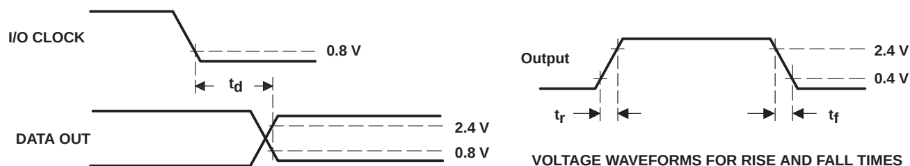
VOLTAGE WAVEFORMS FOR RISE AND FALL TIMES
