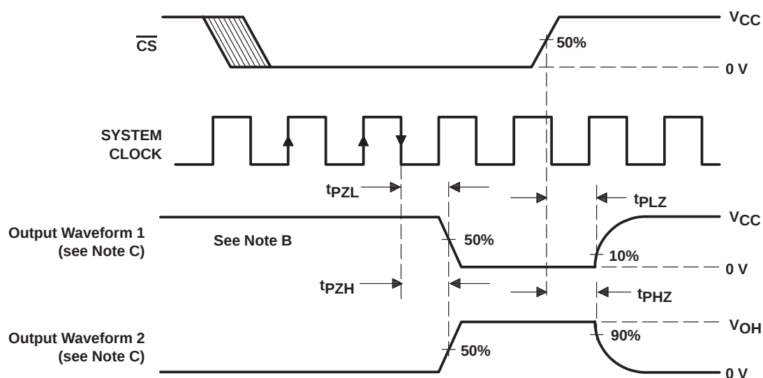
VOLTAGE WAVEFORMS FOR ENABLE AND DISABLE TIMES
